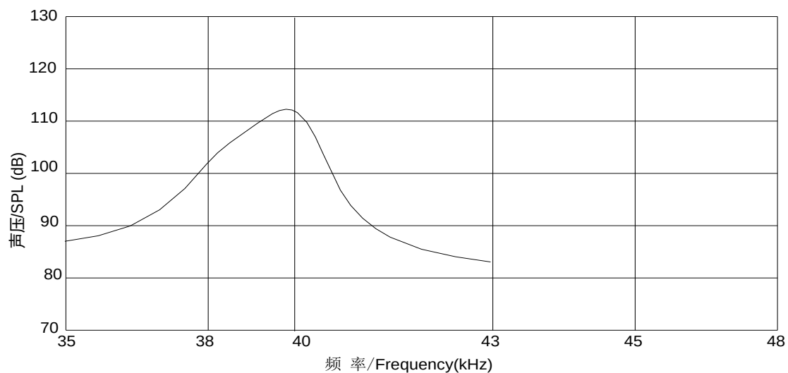
声压-频率特性图/SPL-Frequency Characteristics
